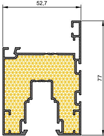
FS - 02 1,344 kg/mt Kanat Profili / Sash Profile
