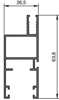
FS - 03 0,678 kg/mt Kanat İç Profili / Sash Inside Profile
