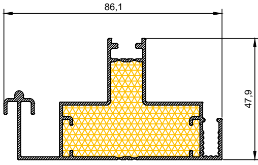
FS - 01 1,130 kg/mt Kasa Profili / Frame Profile
