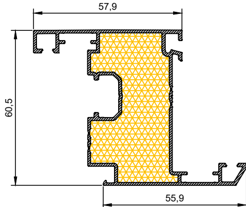
FA - 103 1,135 kg/mt Kanat Profili / Sash Profile
