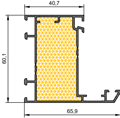
FA - 101 1,036 kg/mt Kasa Profili / Frame Profile
